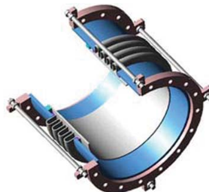
Expansion Joint
